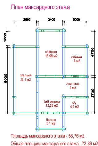
Plan of attic floor
