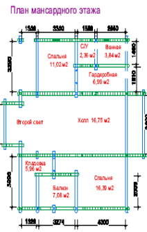
Plan of attic floor
