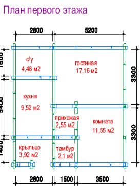
Plane of ground floor
