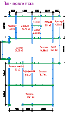
Plane of ground floor
