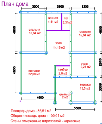
Plan of the house
