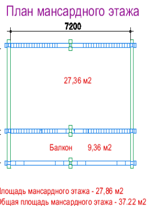
Plan of attic floor
